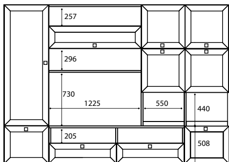
MISURE INTERNE
